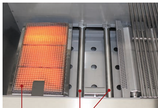
INFRARED BURNER
